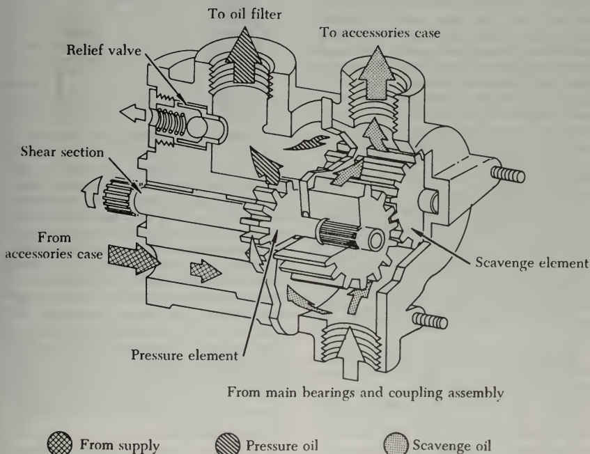
FIGURE 6-24. Cutaway view of gear oil pump.
